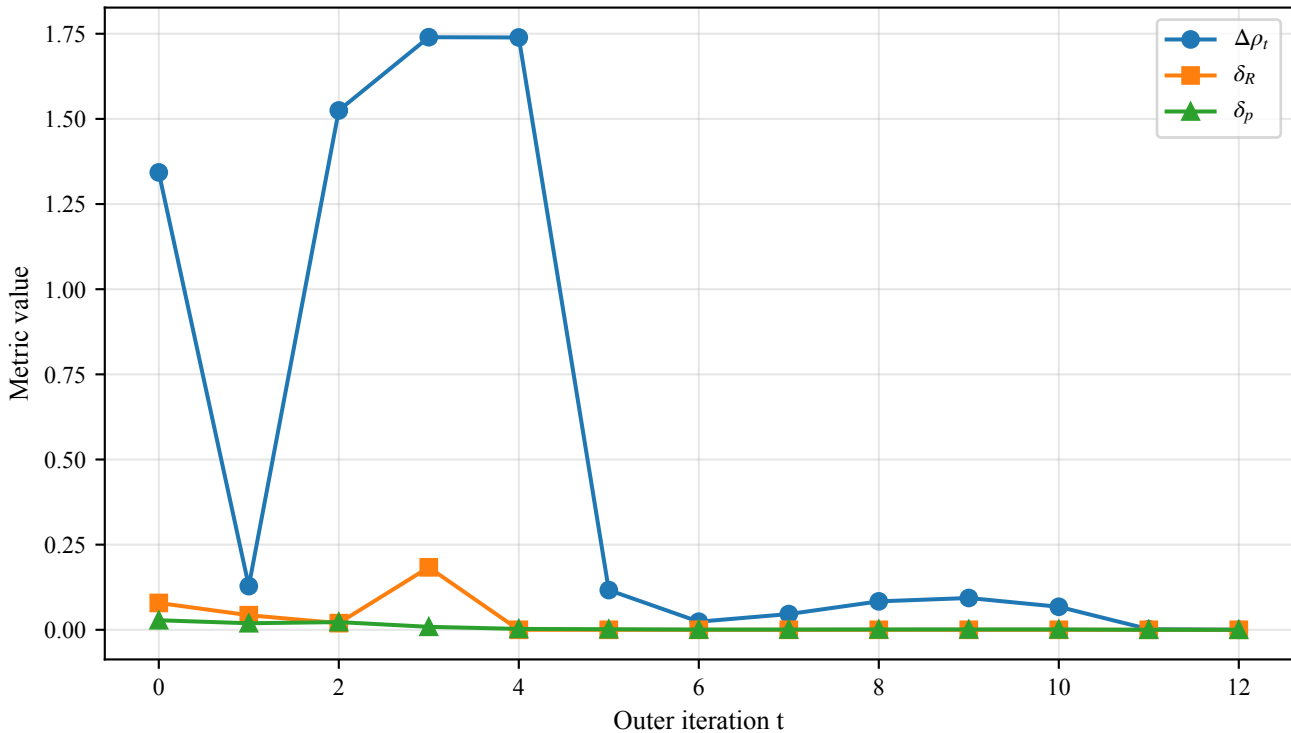
Outer-step diagnostics in Algorithm 2
